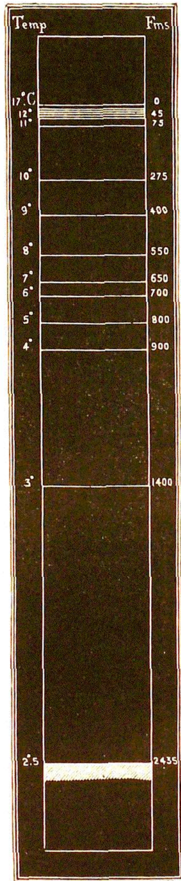
FIG. 60.—Diagram representing the relation between the depth and temperature in the Atlantic basin.
